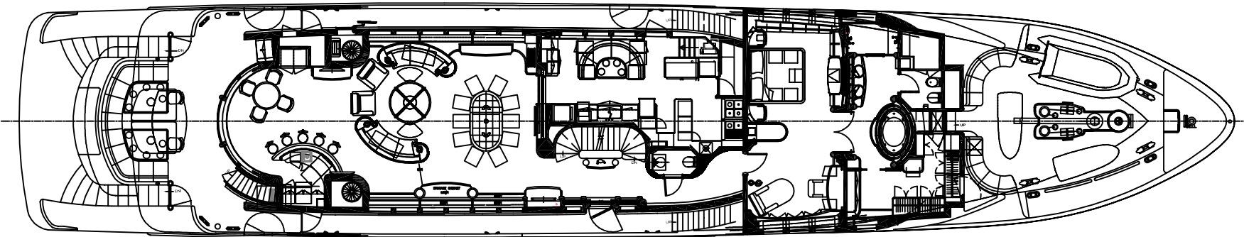
MAIN DECK
