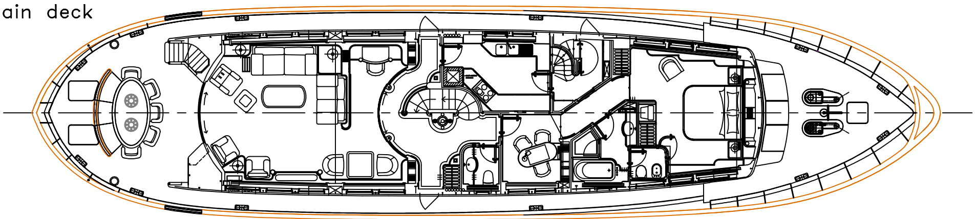
cabin deck
